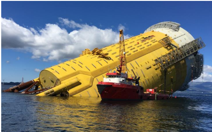
Ballasting operations
